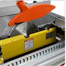
Main and Scoring Blade Assembly
