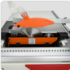
Cutting Unit Assembly, Main and scoring Blade
